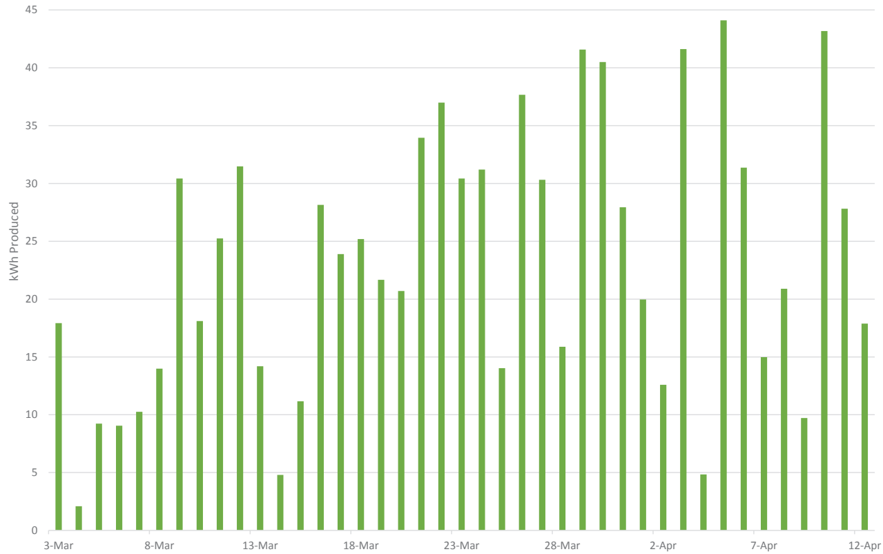
SOLAR OUTPUT FROM 22 PANELS AT BROOKLYN TOWNHOUSE SPRING 2016
